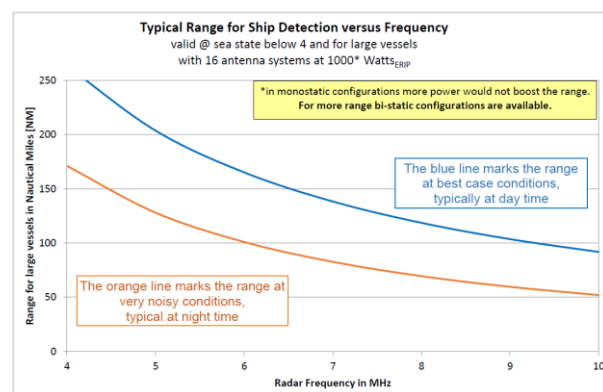
The range for ship detection strongly depends on the operating frequency and is affected by external noise and interference which varies with the day/night cycle.
